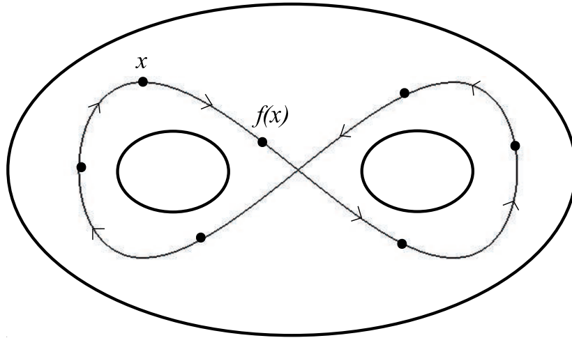
Figure 1: Isotopy loop for a periodic orbit
