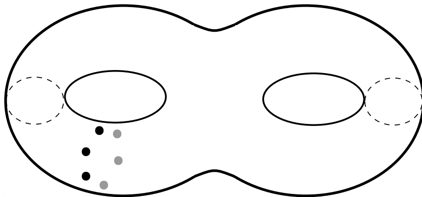
Figure 3: Simple braid on a genus 2 surface
