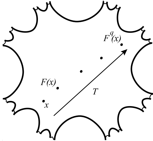
Figure 2: Lift of a surface with boundary
